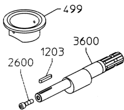
VARIANTES RO 121 TS/1C RESPECTO A RO 106 TS/1C
